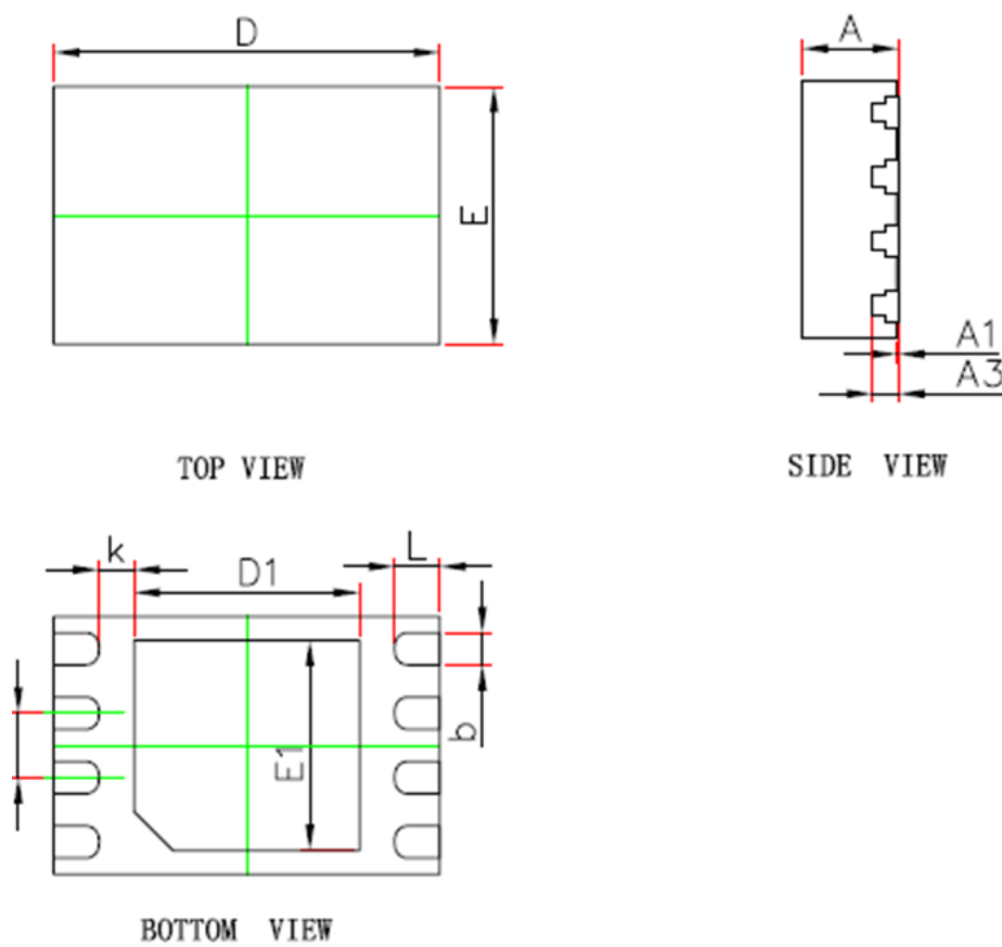
Figure 8. DFN2x3-8L Package, 2 mm x 3 mm Body
