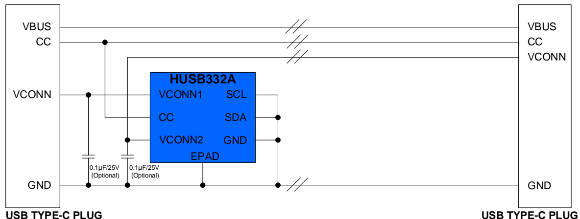
Figure 1.HUSB332A Application Diagram
